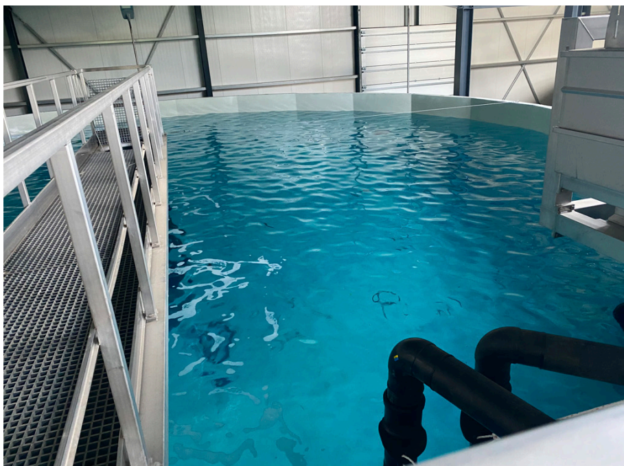
First tank in Kópasker filled with 13,8 °C hot sea water on 9th July 2021, whole year ahead of our plans in Q2 2020. Each tank is equipped with 70% recirculation equipment.
